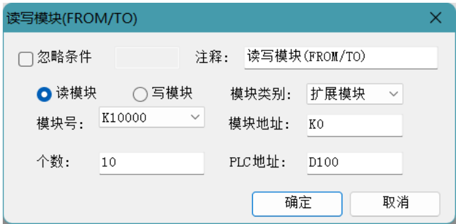
(c) 读模块
