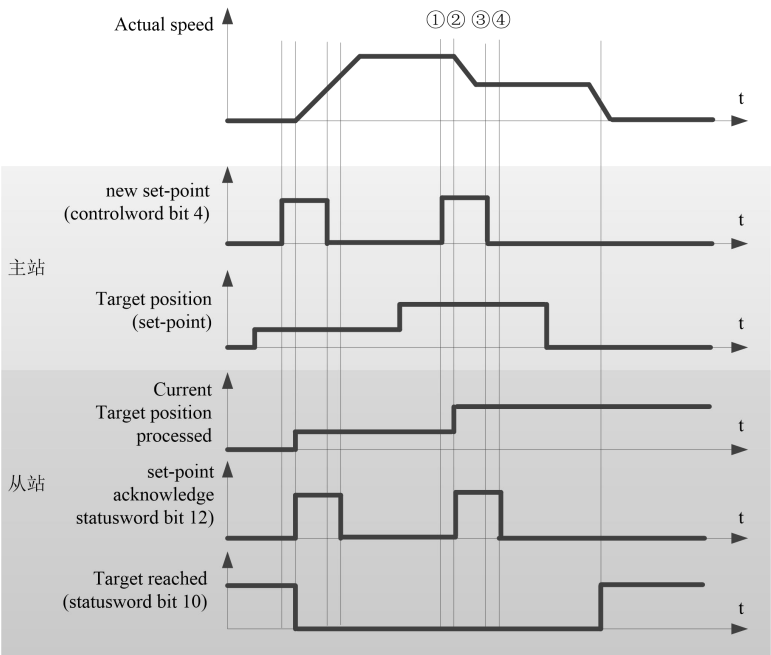
< handshaking procedure for the single set-point method >
